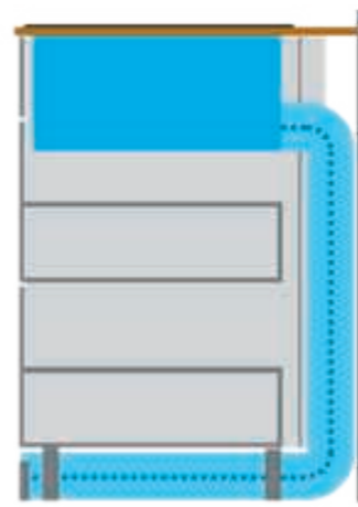
Maximum Drawer Depth 513mm with 70+cm worktop
