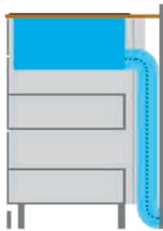
Maximum Drawer Depth 513mm with 70+ worktop
