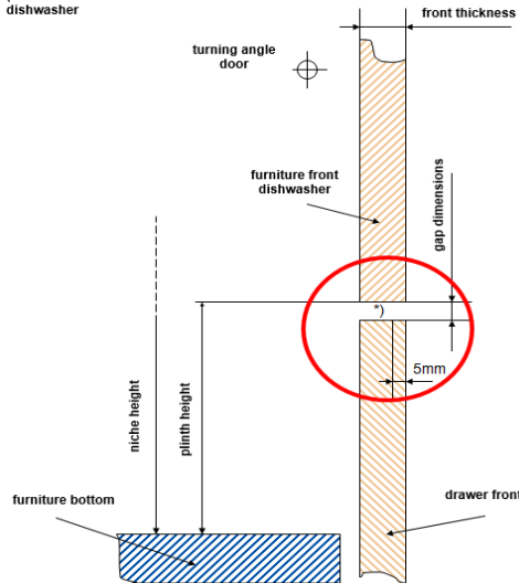
High Installation of BSH Dishwashers - Drawing (without bevel of furniture front below the dishwasher)
