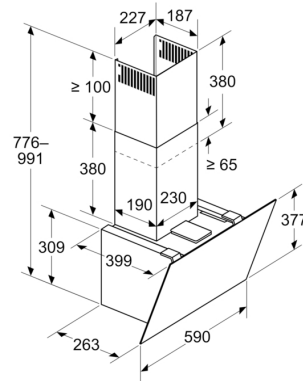
Measurements in mm Appliance in circulated air mode
