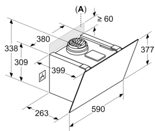
Measurements in mm Appliance in circulated air mode without duct
