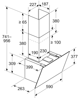
Measurements in mm Appliance in exhaust air mode
