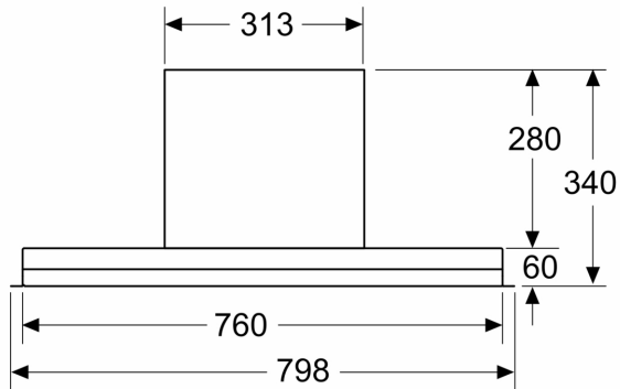
Measurements in mm Front view
