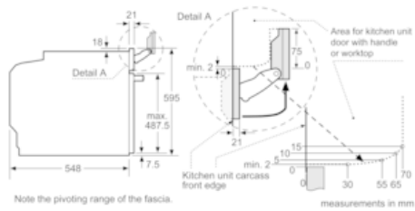
Dimensioned drawings
